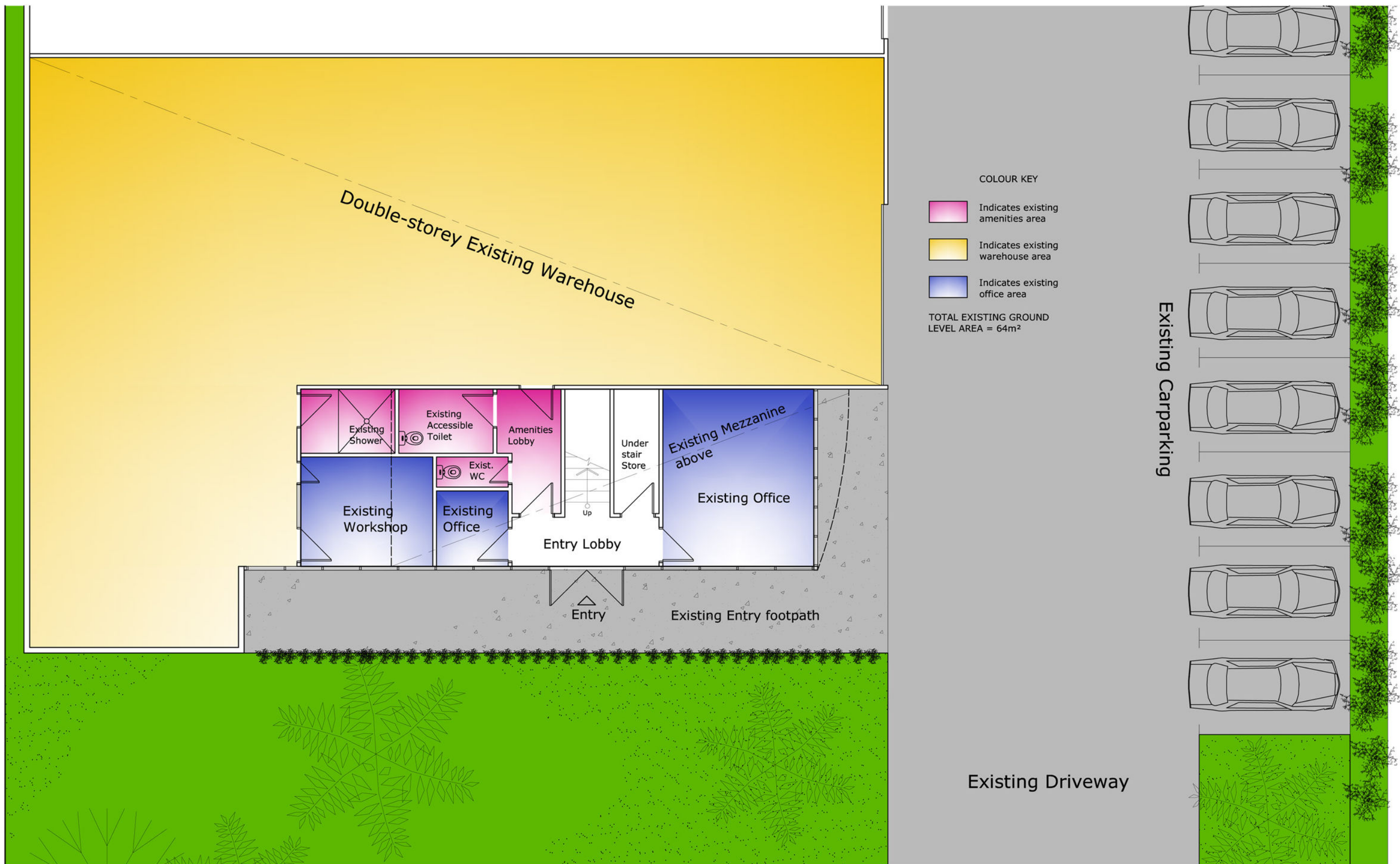
1 EXISTING GROUND LEVEL PLAN SCALE: 1:100 @ A3/1:50 @ A1
