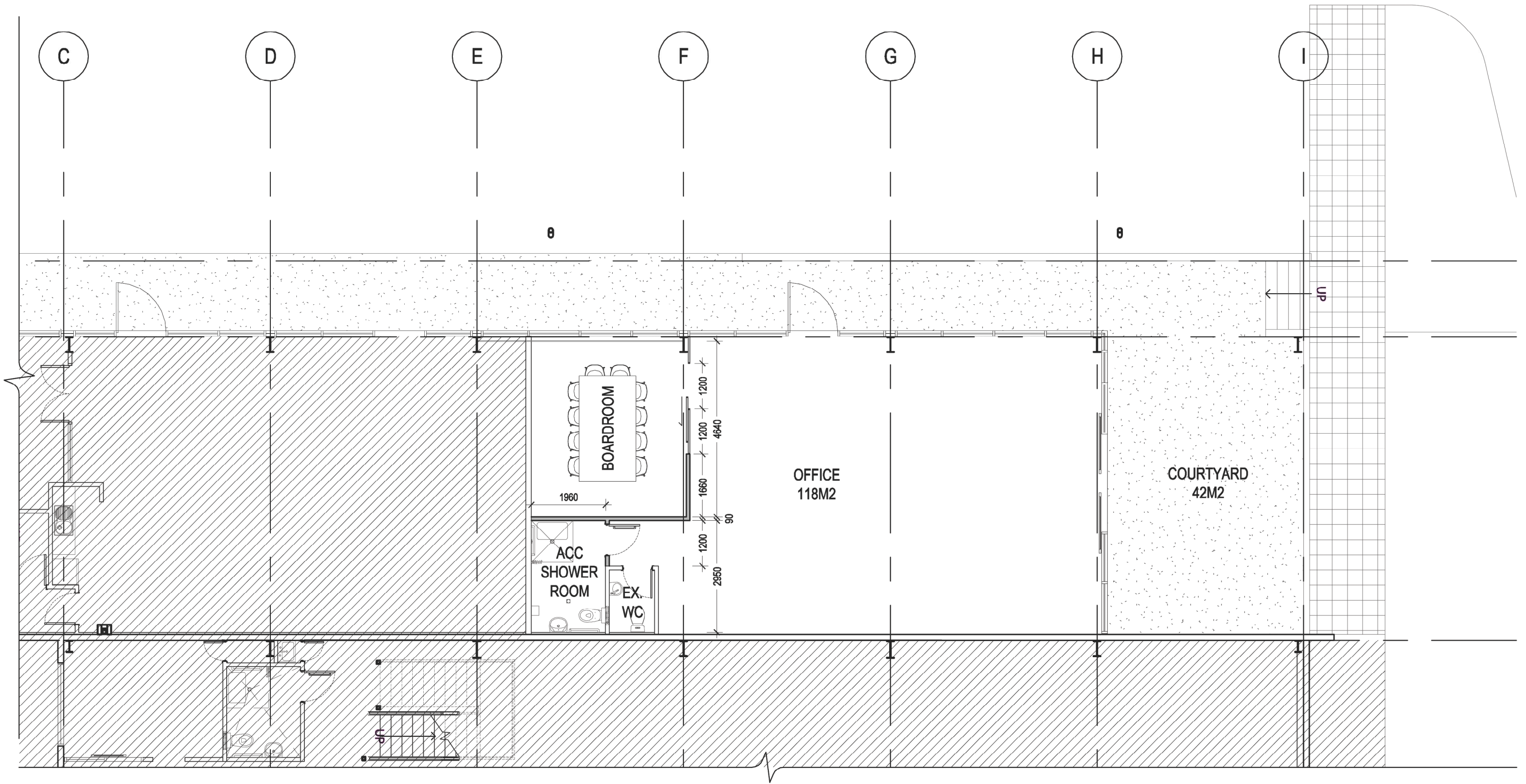
01 PROPOSED FLOOR PLAN 1:100 © A3
